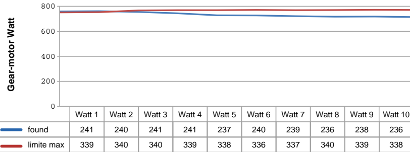
clockwise rotation Watt
